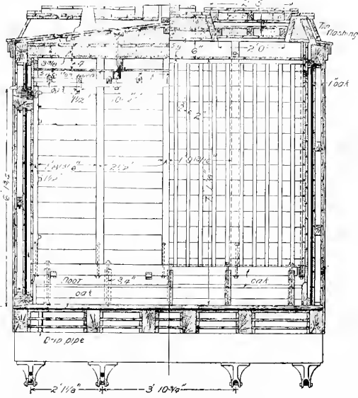
Fig. 277. Transverse Sections.
